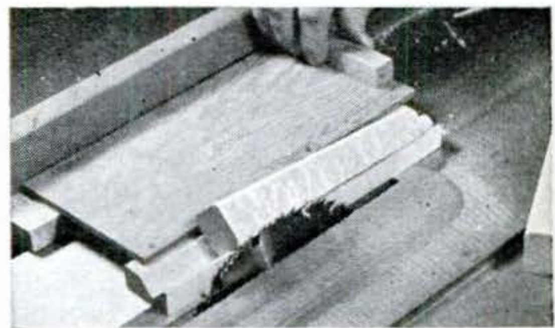
V ATTACHMENT IS SUBSTITUTED for the notched guide strip for cutting chamfers on the tapering corners. Work should be held down lightly to prevent vibration.
